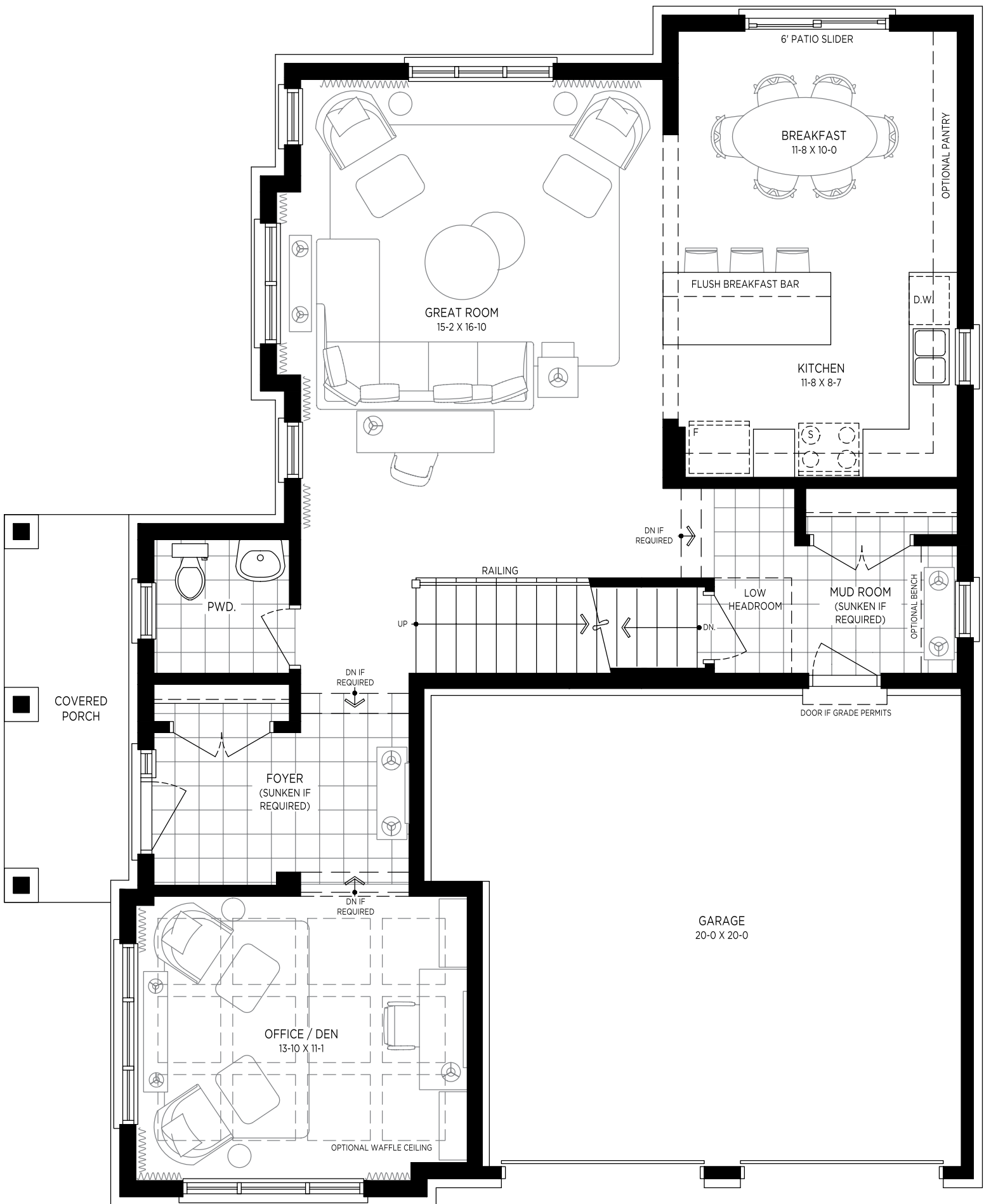
MAIN FLOOR PLAN 'A'
